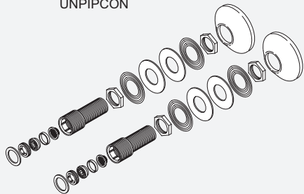
Straight inlet connector (pair) UNPIPCON
