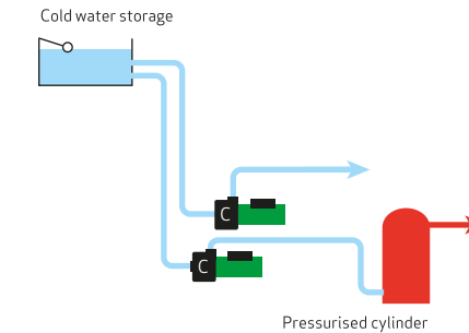
Figure 12: Pressurised cylinder or Combination boiler system
